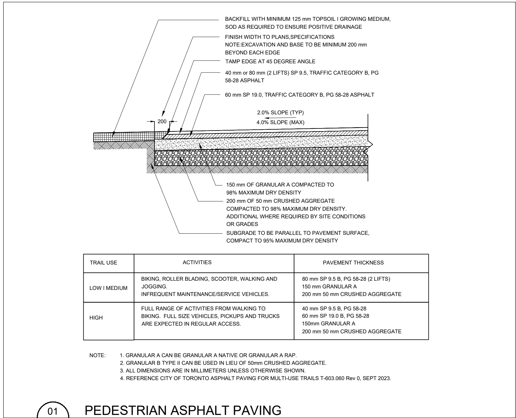
01 0001 PEDESTRIAN ASPHALT PAVING DETAIL
