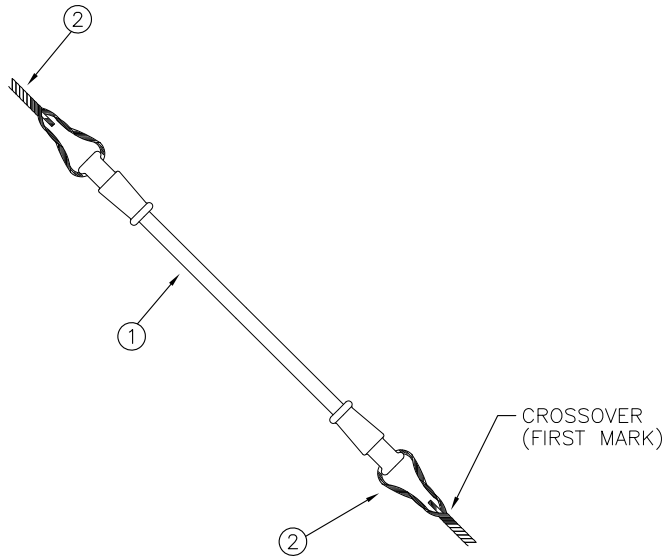
FIG. 1 GUY INSULATOR
