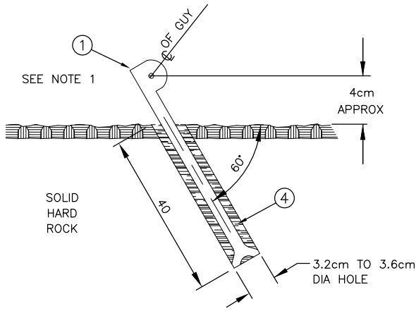
FIG. 1 ROCK ANCHOR
