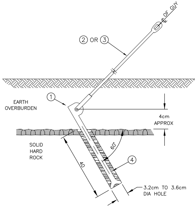
FIG. 2 ROCK ANCHOR WITH EARTH OVERBURDEN
