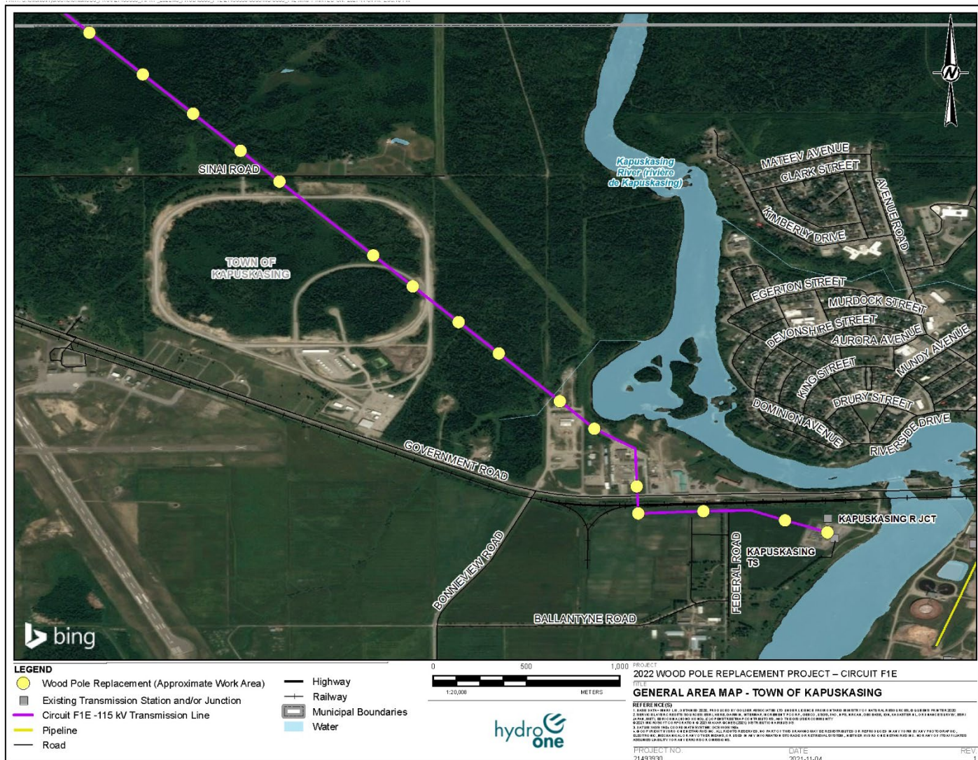
Map of project area for wood pole replacement on Circuit F1E within the Town of Kapuskasing:
