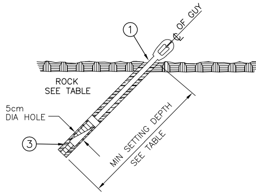
FIG. 1 EXPANDING ROCK ANCHOR
