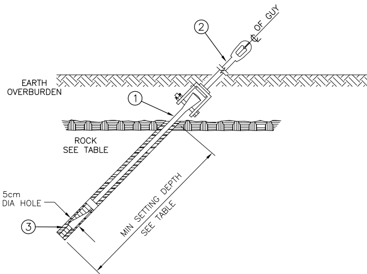
FIG. 2 EXPANDING ROCK ANCHOR WITH EARTH OVERBURDEN
